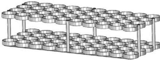
Part No. 2111 Model M6-4000 Dim: 8.375"Hx15.5"Wx38.75"L Zinc Plated
