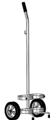
Part No. 4050 Model: ML6-2 Holds 2 ML6 or M7 cyl Dim: 38"Hx14"Wx11"D Chrome Plated
